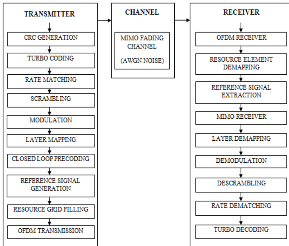
Fig. 2. System Model of LTE Downlink
