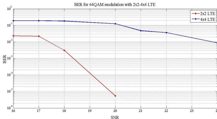
Fig. 4. BER vs. SNR plot for 2x2-4x4 LTE with 64QAM modulation for RAYLEIGH fading
