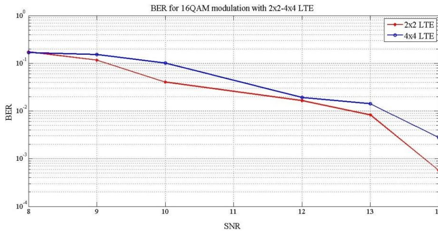
Fig. 3. BER vs. SNR plot for 2x2-4x4 LTE with 16QAM modulation for RAYLEIGH fading
